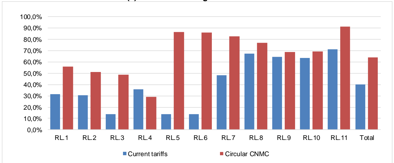
Figure 12. Proportion of the billing of the capacity term of the current tariffs and of the tariffs of the Circular (1) recovered through the fixed term. Year 2020.
